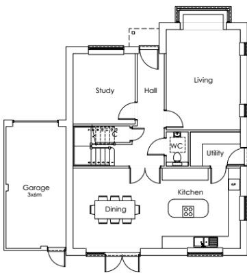
Ground Floor Plan 1:100
