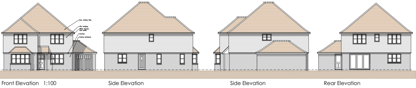
Front Elevation 1:100
